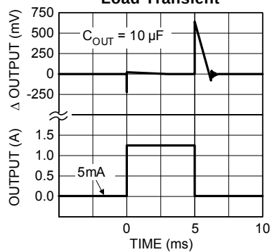
Load Transient
