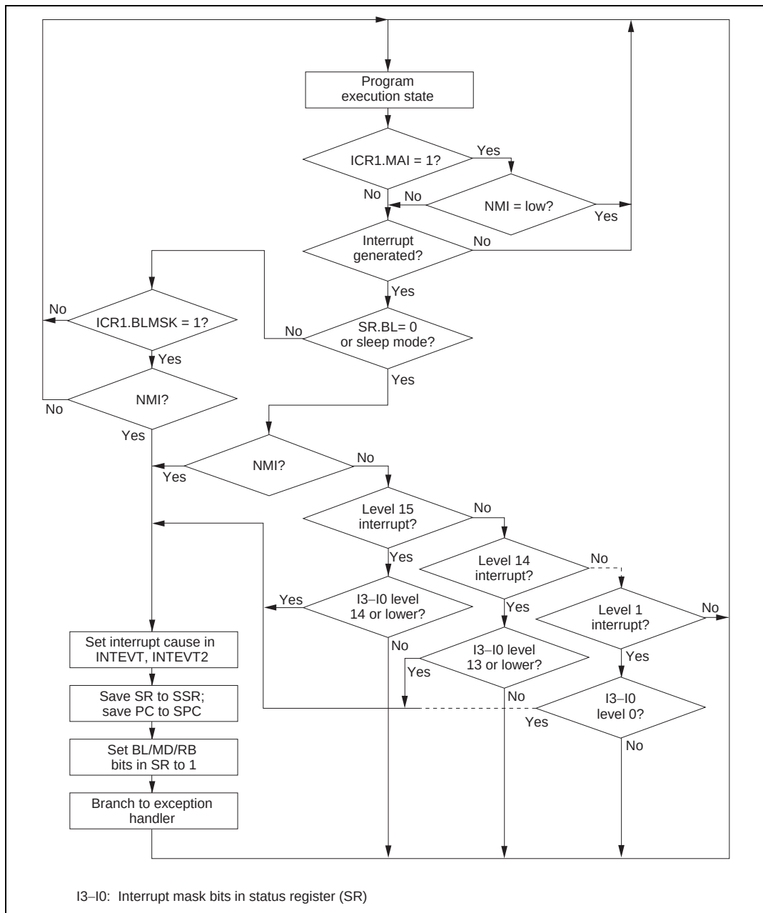
Figure 7.3 Interrupt Operation Flowchart
