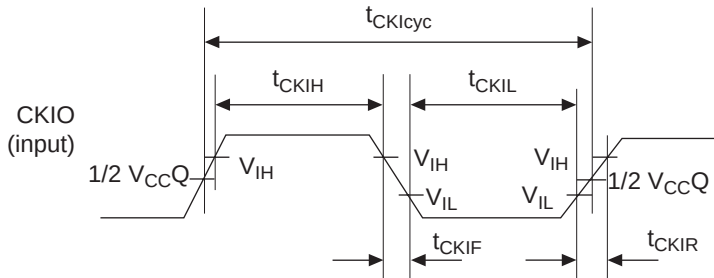
Figure 32.4 CKIO Clock Input Timing
