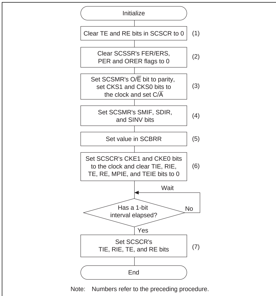
Figure 18.5 Initialization Flowchart (Example)
