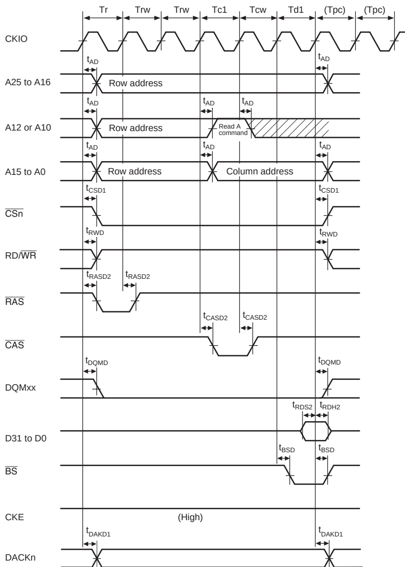
Figure 32.24 Synchronous DRAM Read Bus Cycle (RCD = 2, CAS Latency = 2, TPC = 1)
