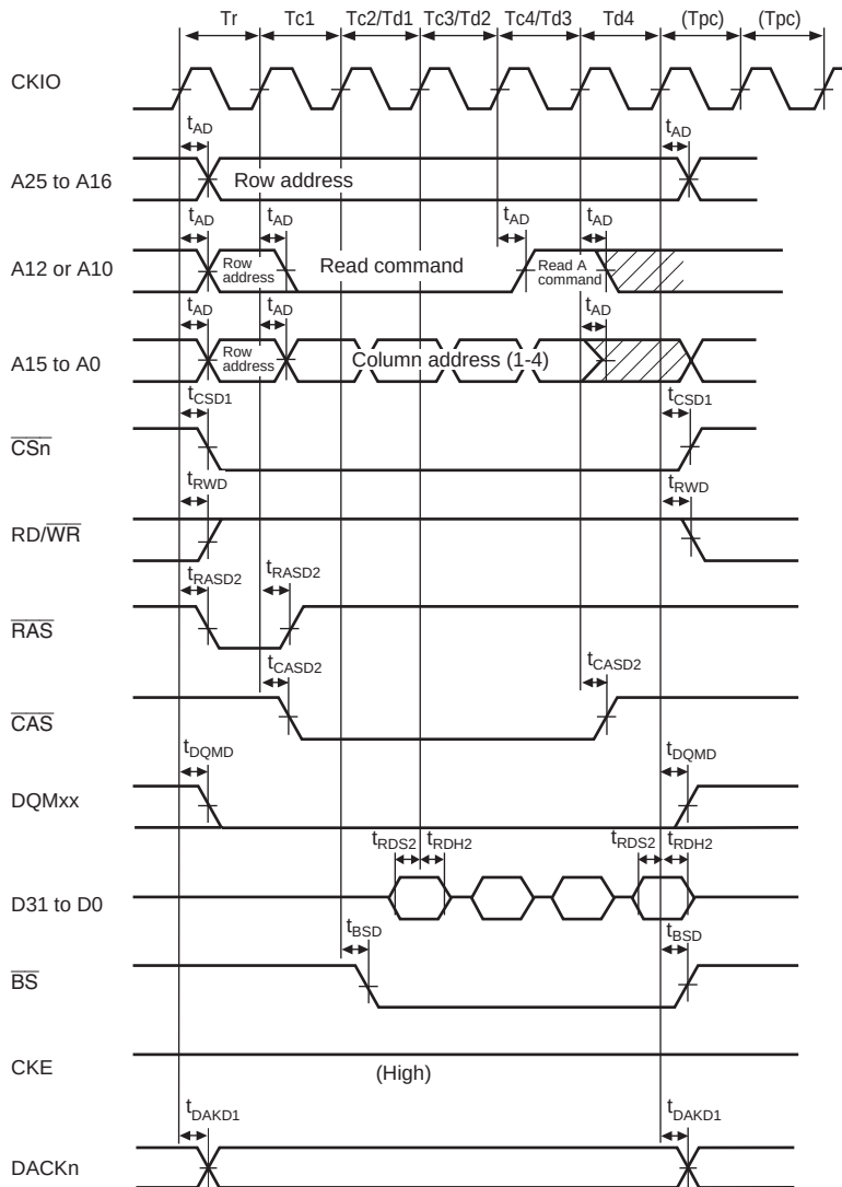
Figure 32.25 Synchronous DRAM Read Bus Cycle (Burst Read (Single Read \times 4), RCD = 0, CAS Latency = 1, TPC = 1)
