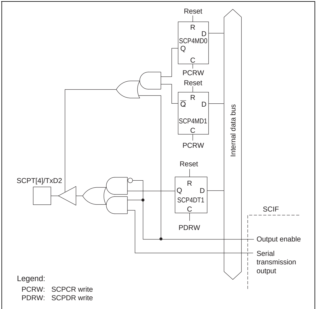
Figure 19.2 SCPT[4]/TxD2 Pin
