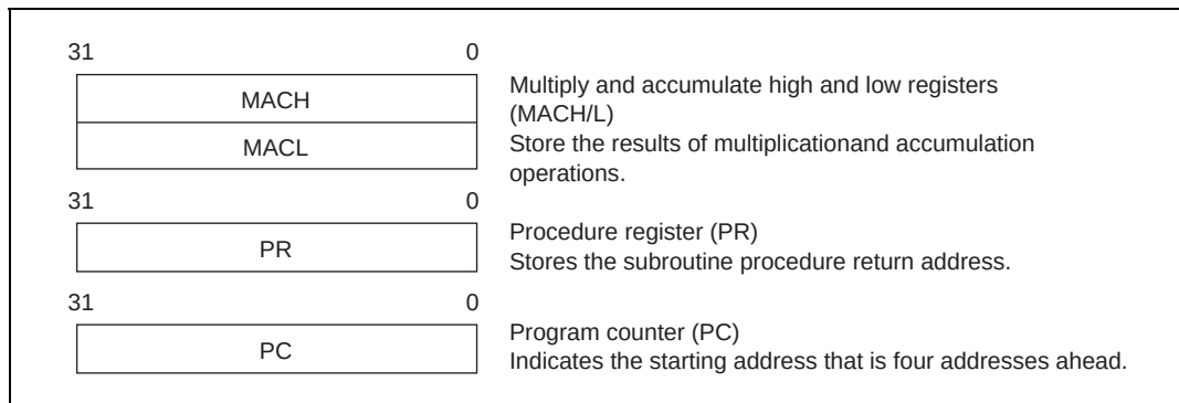
Figure 2.6 System Registers
