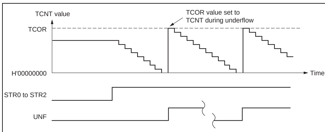
Figure 15.3 Auto-Reload Counter Operation
