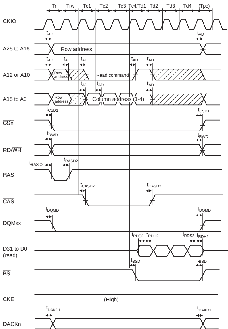
Figure 32.26 Synchronous DRAM Read Bus Cycle (Burst Read (Single Read x 4), RCD = 1, CAS Latency = 3, TPC = 0)
