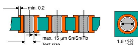
Plated-through bore hole with Sn/SnPb
