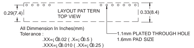
Figure 8. Recommended VPOL10A-12W-SIP Footprint
