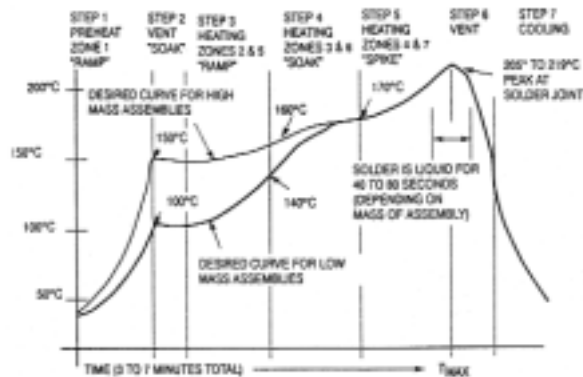
Typical Soldering Heating Profile
