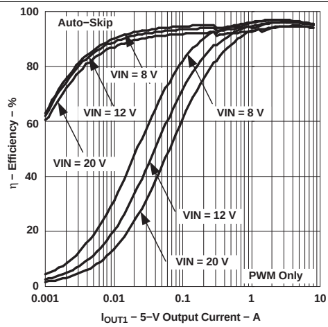
Figure 25. 5-V Efficiency vs Output Current
