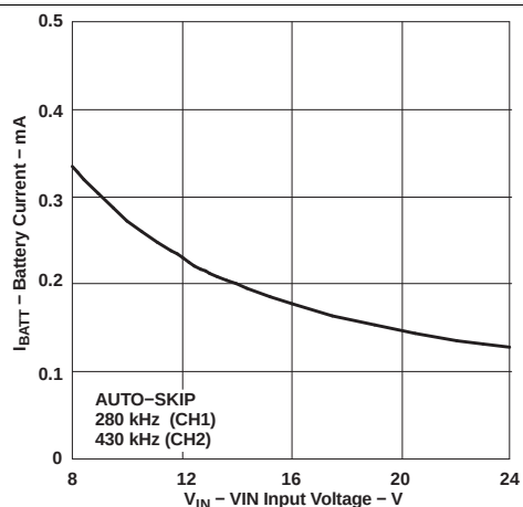
Figure 7. No-Load Battery Current vs Input Voltage
