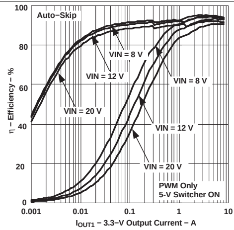
Figure 26. 3.3-V Efficiency vs Output Current
