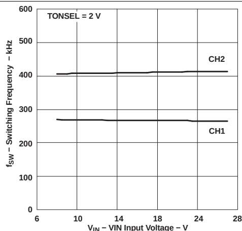
Figure 10. Switching Frequency vs Input Voltage
