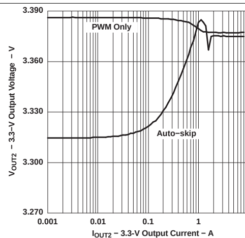
Figure 22. 3.3-V Output Voltage vs Output Current
