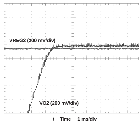
Figure 38. 3.3-V Switchover Waveforms
