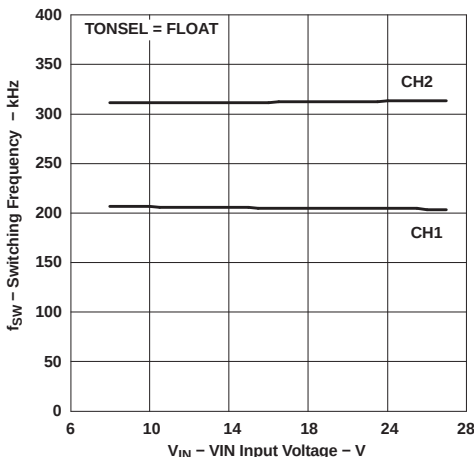
Figure 11. Switching Frequency vs Input Voltage
