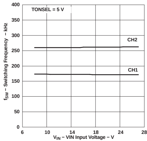
Figure 12. Switching Frequency vs Input Voltage
