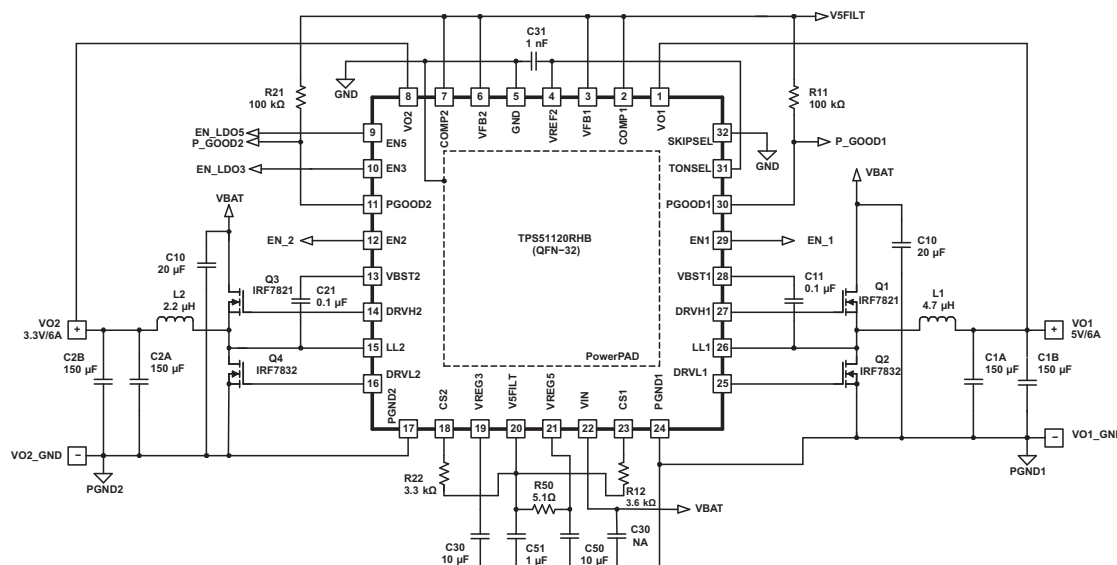
Reference Design for D-CAP Mode Converter
