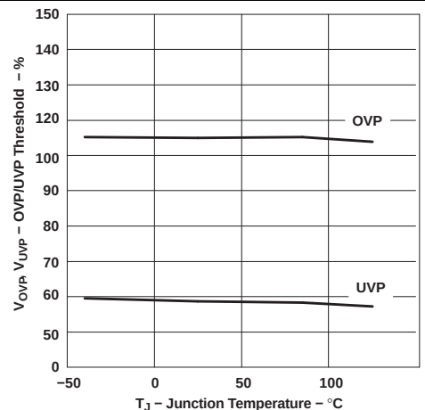
Figure 17. OVP/UVP Threshold Voltage vs Junction Temperature
