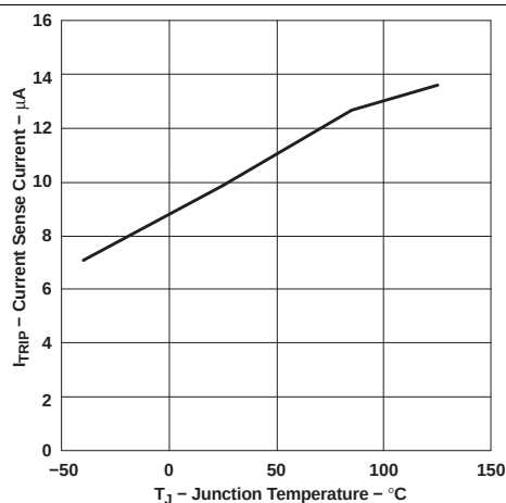
Figure 8. Current Sense Current vs Junction Temperature
