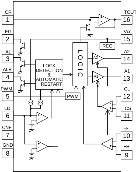
Fig.2 Block diagram
