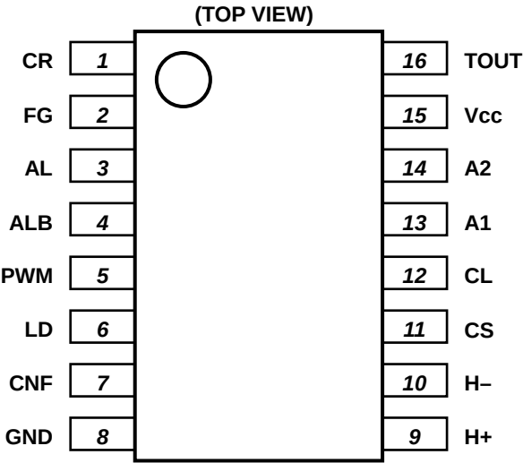
Fig. 1 Pin configuration
