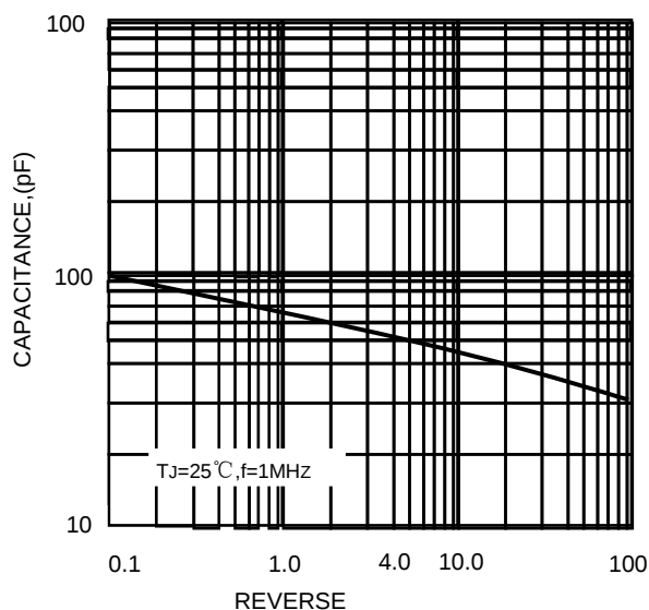
FIG.3-TYPICAL JUNCTION
