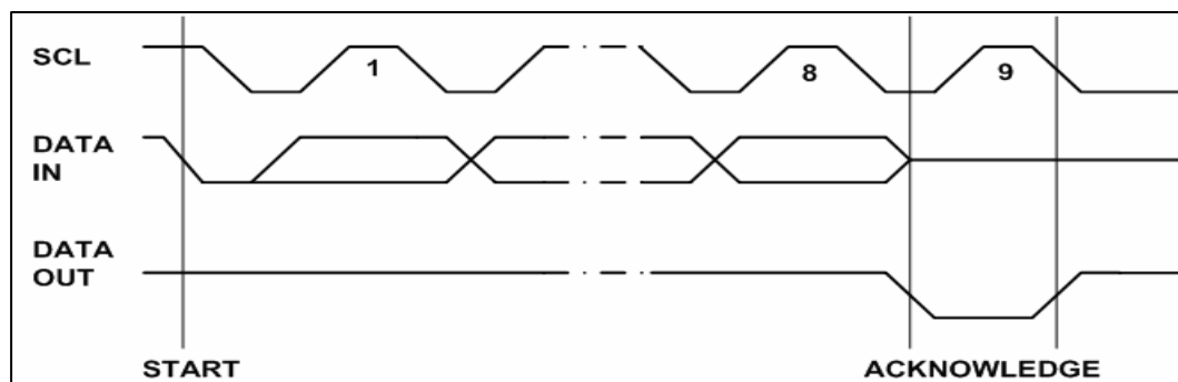
Figure 6 · Output Acknowledge
