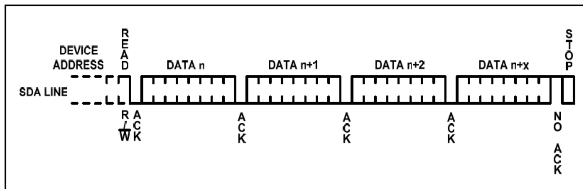
Figure 12 · Sequential Read
