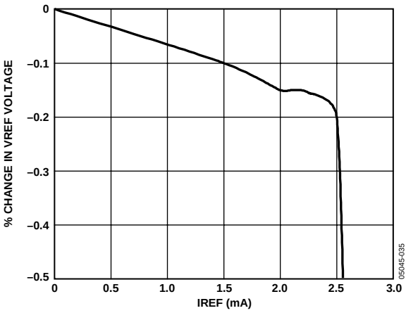
Figure 34. Internal VREF vs. Load Current
