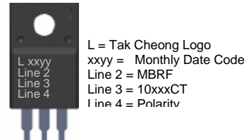
TO-220FP
