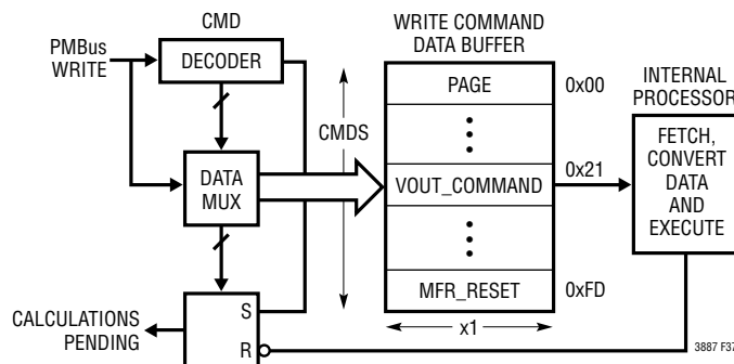
Figure 37. Write Command Data Processing
