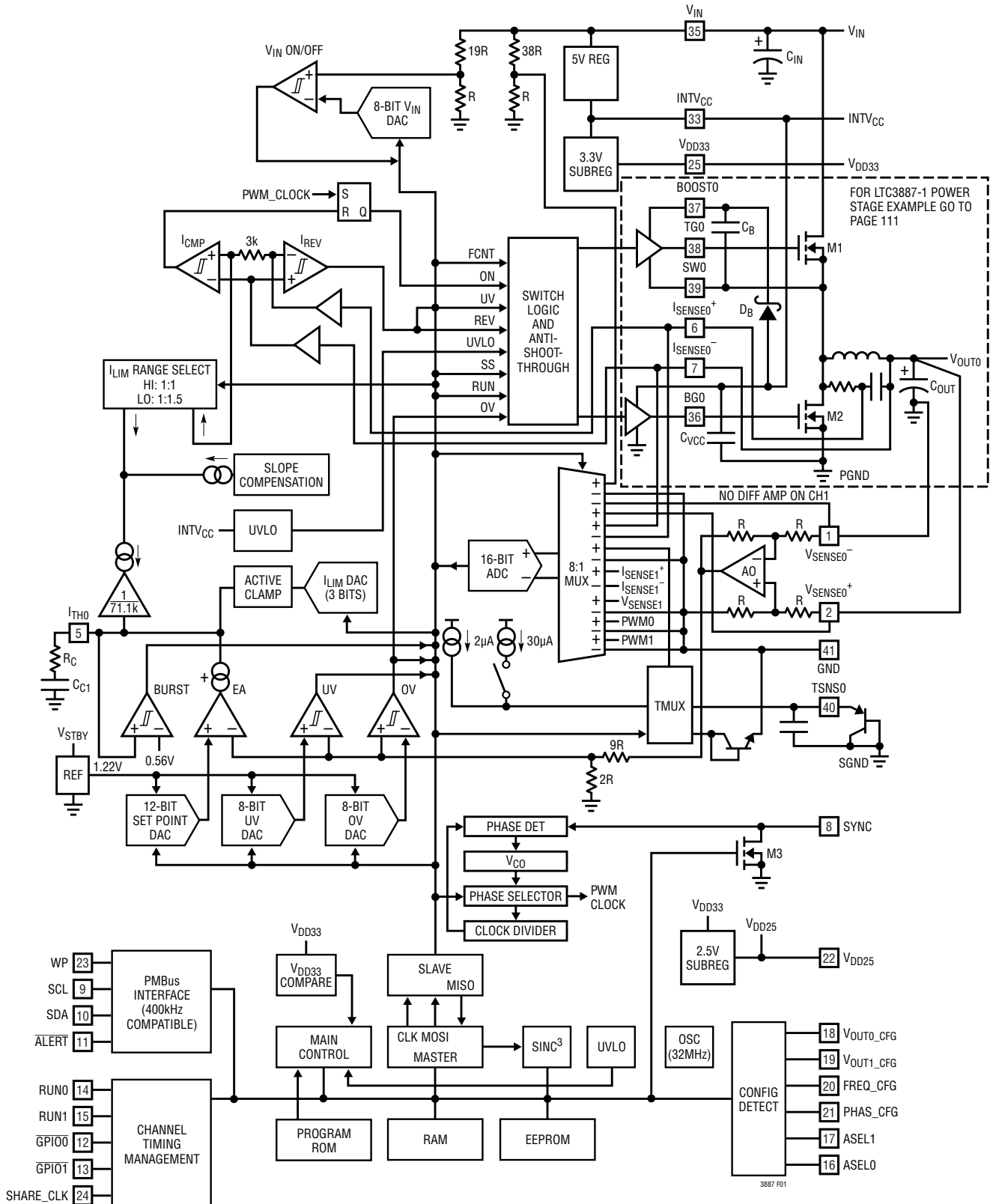
Figure 1. Block Diagram
