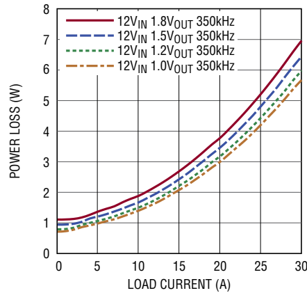
Power Loss vs Load Current F SW = 350kHz (LTC3887)
