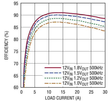
Efficiency vs Load Current F SW = 500kHz (LTC3887)
