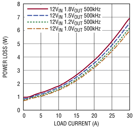
Power Loss vs Load Current F SW = 500kHz (LTC3887)
