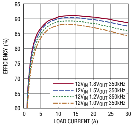
Efficiency vs Load Current F SW = 350kHz (LTC3887)
