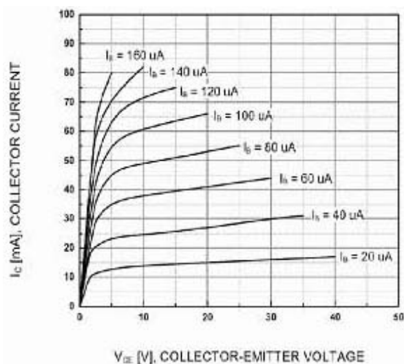
Static Characteristic
