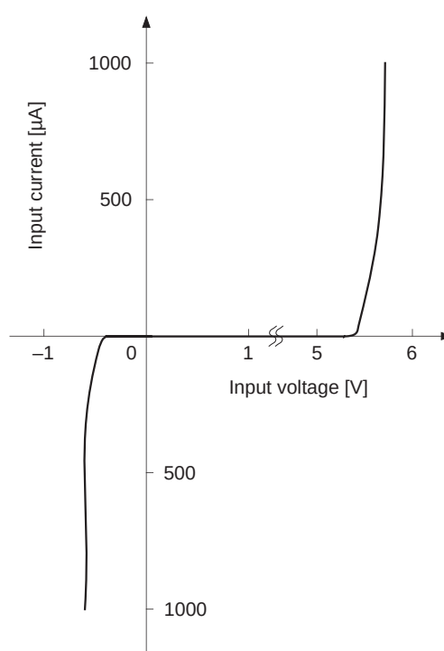
Fig. 10. Input terminal V-I characteristics
