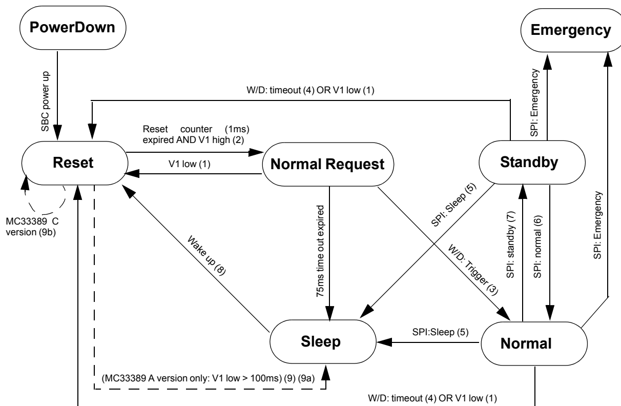
Figure 20. State Machine
