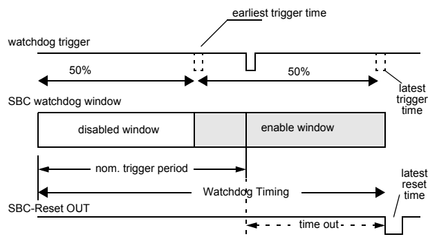
Figure 15. Window Watchdog Timing
