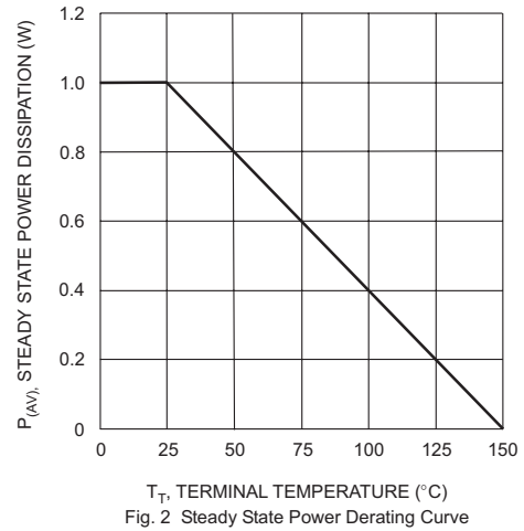
Fig. 2 Steady State Power Derating Curve
