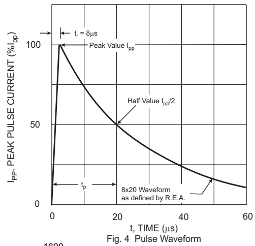
Fig. 4 Pulse Waveform
