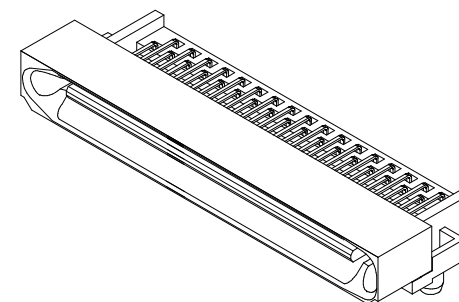
68 CIRCUIT ASSEMBLY SHOWN SCALE 2:1
