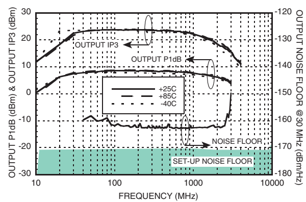
Output IP3, P1dB & Noise Floor @ 30 MHz Offset vs. Frequency
