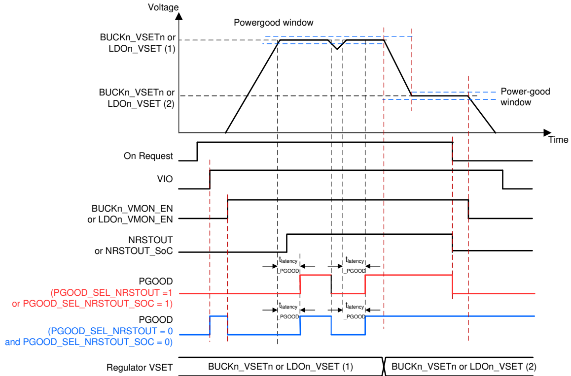
Figure 8-12. PGOOD Waveforms
