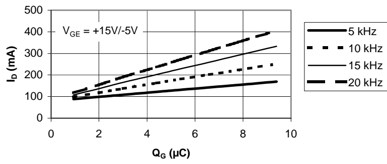
Figure 6 Supply Current versus Gate Charge
