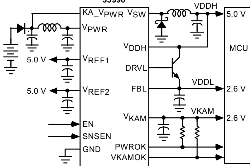
33998 Simplified Application Diagram 33998
