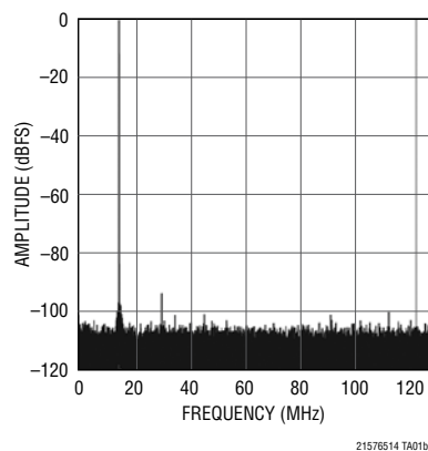
LTC2157-14 32K Point FFT, f_{\text{IN}} = 15\text{MHz} , -1dBFS, 250Msps
