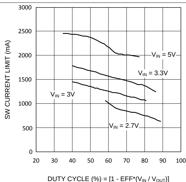
Figure 29. Switch Current Limit vs Duty Cycle - Y Option
