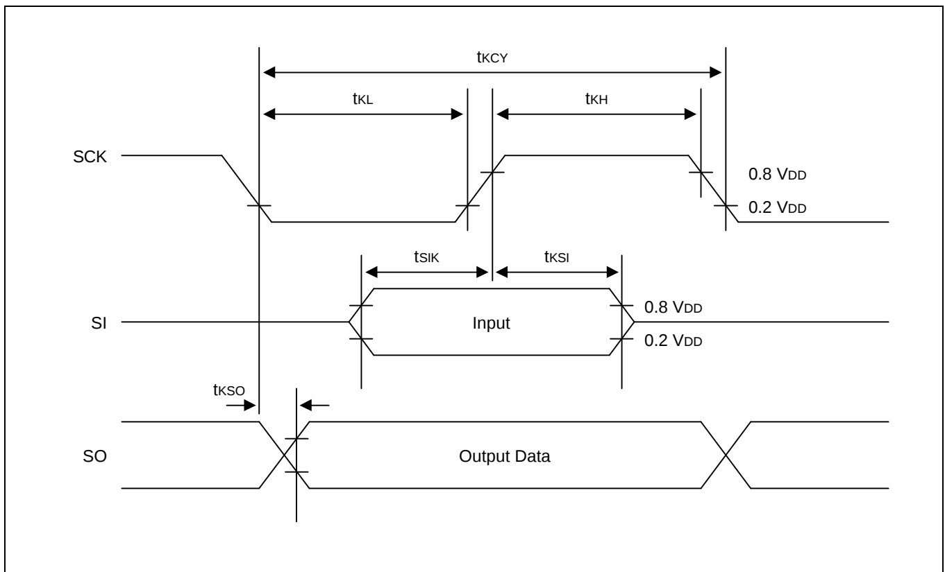
Figure 14-6. Serial Data Transfer Timing
