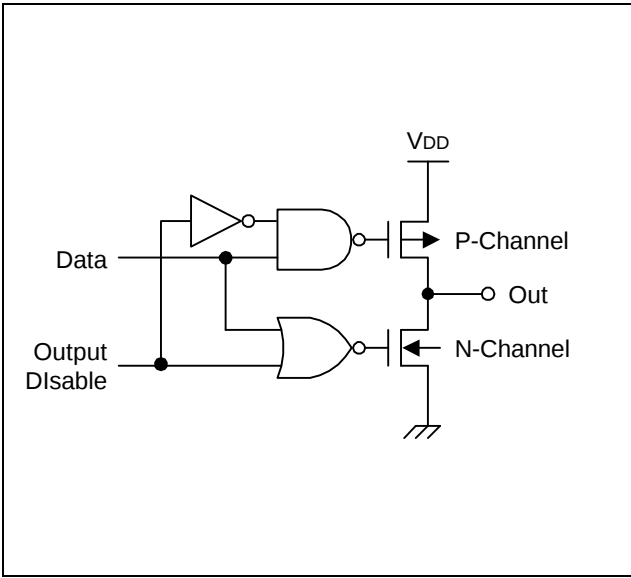
Figure 1-8. Pin Circuit Type C
