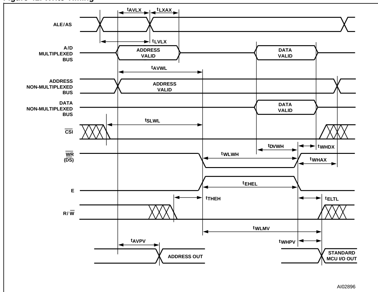
Figure 42. Write Timing
