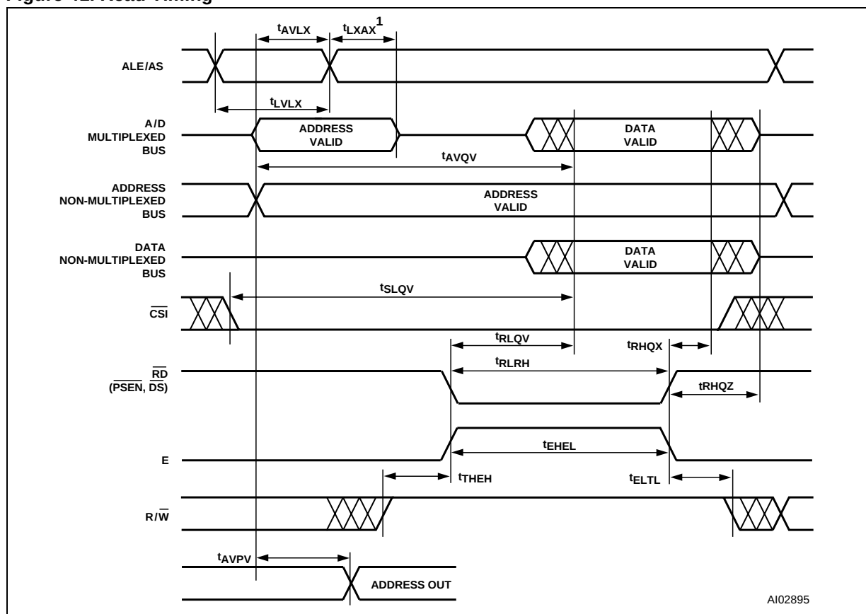
Figure 41. Read Timing
