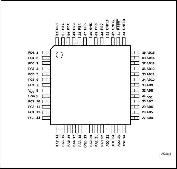
Figure 48. PQFP Connections
