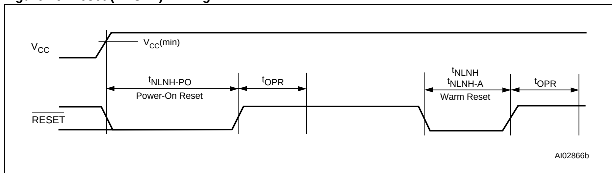
Figure 45. Reset ( \overline{RESET} ) Timing
