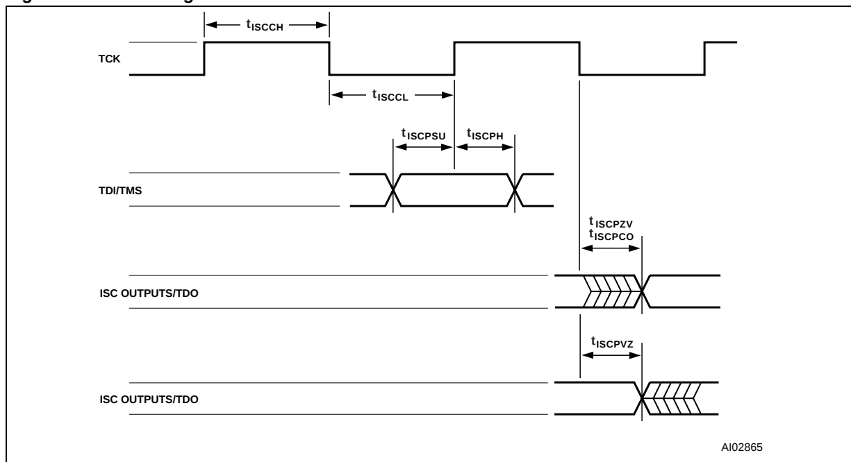
Figure 46. ISC Timing
