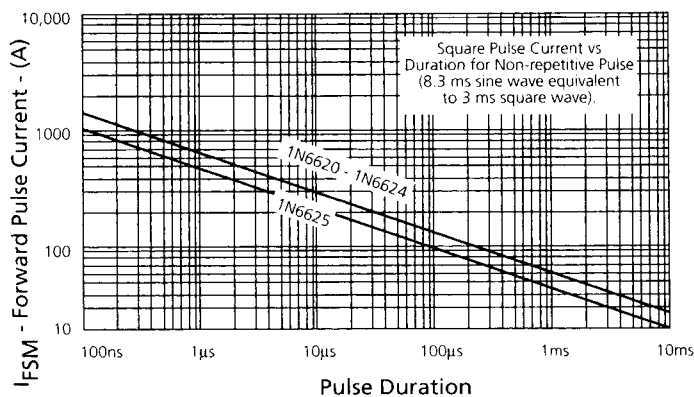
FIGURE 7 Forward Pulse Current vs. Pulse Duration
