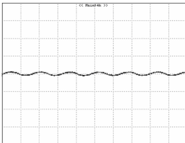
Figure 11: Input Terminal Ripple Current, i_c , at 48Vin and 20 output current with 12\mu H source impedance and 33\mu F electrolytic capacitor (500 mA/div, 2us/div).
