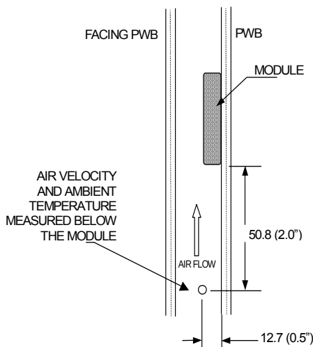
Figure 20: Wind tunnel test setup
