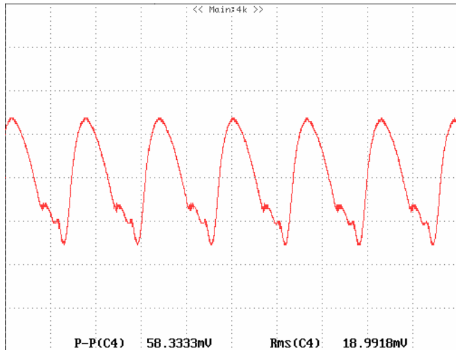
Figure 14: Output voltage ripple at 48\text{V}_{\text{in}} and rated load current ( I_o=20\text{A} ) (20 mV/div, 2\mu\text{s}/\text{div} ) Load capacitance: 1\mu\text{F} ceramic capacitor and 10\mu\text{F} tantalum capacitor. Bandwidth: 20 MHz.
