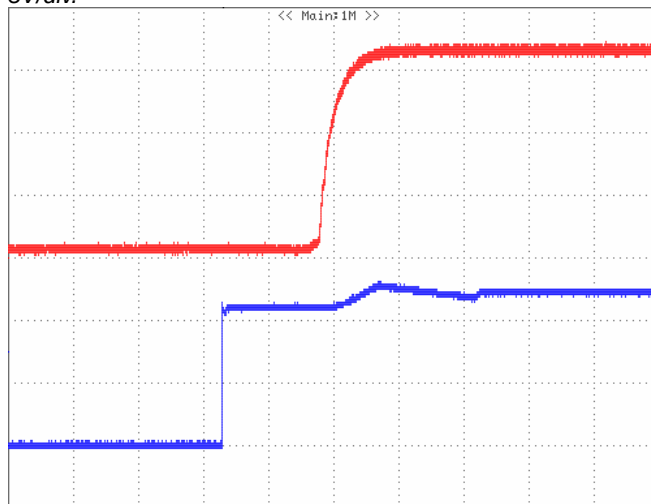
Figure 7: Turn-on transient at zero load current (5ms/div). V_{in}=48V . Top Trace: V_{out} , 2V/div; Bottom Trace: input voltage, 20V/div.
