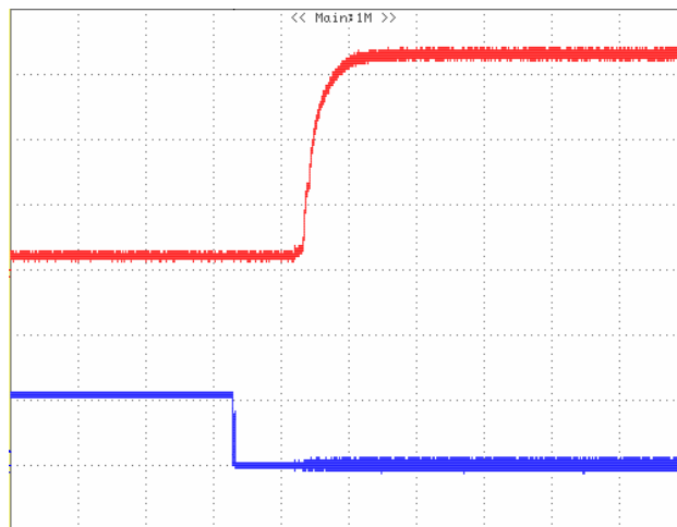
Figure 5: Turn-on transient at zero load current (5ms/div). V_{in}=48V . Top Trace: V_{out} , 2V/div; Bottom Trace: ON/OFF input, 5V/div.
