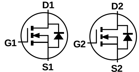
Equivalent Circuit
