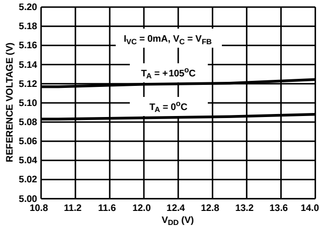
FIGURE 9. TYPICAL REFERENCE VOLTAGE vs SUPPLY VOLTAGE FOR 0^\circ\text{C} AND +105^\circ\text{C}
