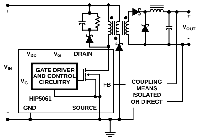
FIGURE 41. FORWARD CONVERTER
