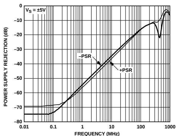
Figure 46. Power Supply Rejection vs. Frequency
