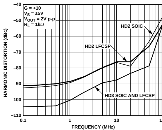
Figure 23. Harmonic Distortion vs. Frequency for Various Packages
