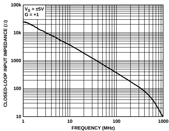
Figure 48. Input Impedance vs. Frequency
