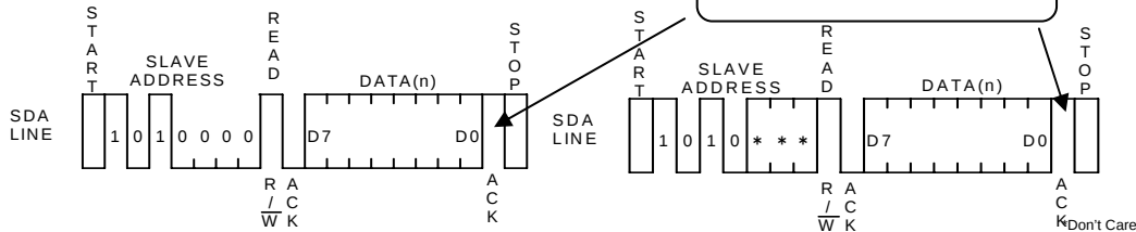
Fig.42 Current read cycle (port1 EEPROM)
