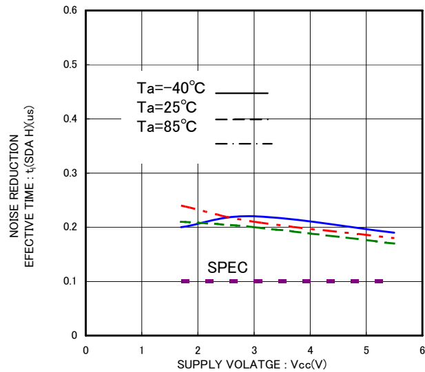
Fig.30 Noise reduction effective time t_1(\text{SDA H})
