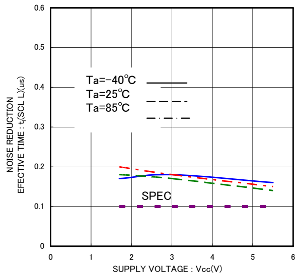
Fig.29 Noise reduction effective time t_1(\text{SCL L})
