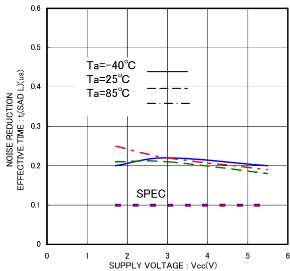
Fig.31 Noise reduction effective time t_1(\text{SDA L})
