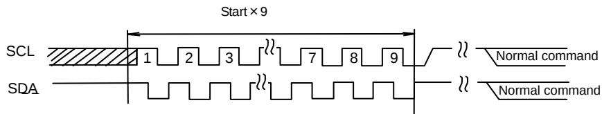
Fig.48 START x 9 + command input
