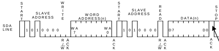
Fig.40 Random read cycle (port1 EEPROM)
