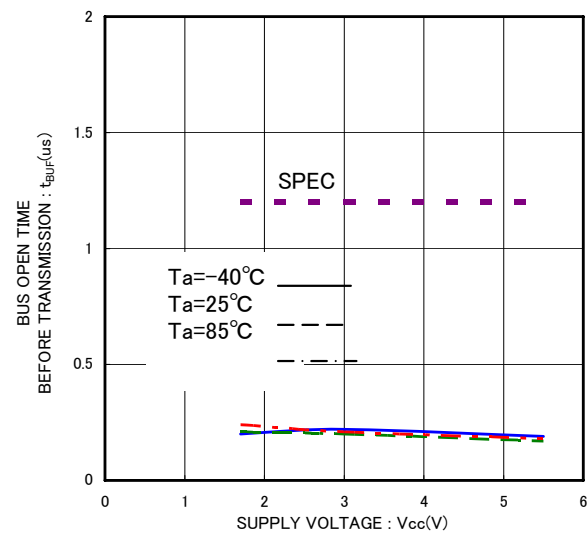
Fig.26 BUS open time before transmission t_{BUF}
