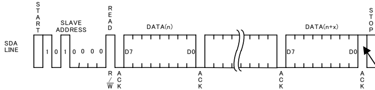
Fig.44 Sequential read cycle (port1 EEPROM)
