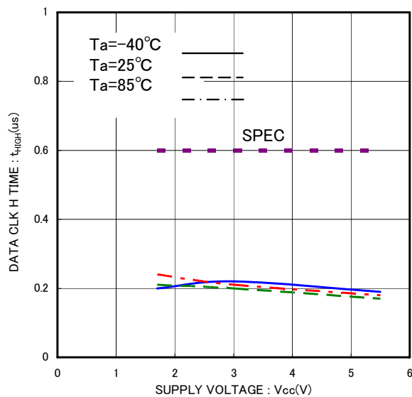
Fig.15 Data clock High Period t_{HIGH}
