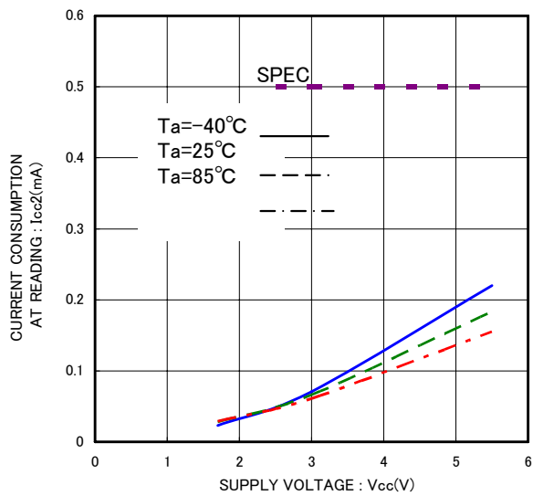
Fig.12 Current consumption at READ operation I_{CC2} (fsc1=400kHz)
