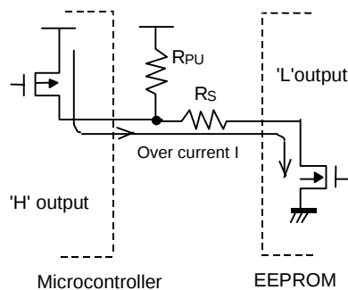
Fig.54-(b) I/O circuit diagram
