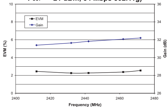
Figure 3: EVM and Gain vs. Frequency ( T_A = +25^\circ\text{C} , V_{CC} = +3.3\text{ V} , V_{REF} = +2.85\text{ V} , P_{OUT} = +21\text{ dBm} , 54 Mbps 802.11g)
