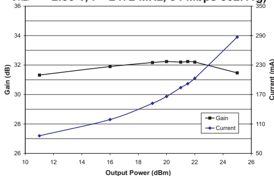
Figure 5: Gain and Current Consumption vs. Output Power ( T_A = +25^\circ\text{C} , V_{CC} = +3.3\text{ V} , V_{REF} = +2.85\text{ V} , f = 2472\text{ MHz} , 54 Mbps 802.11g)
