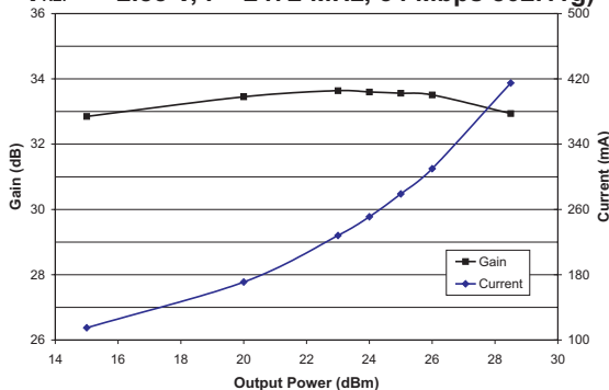
Figure 6: Gain and Current Consumption vs. Output Power ( T_A = +25^\circ\text{C} , V_{CC} = +5\text{ V} , V_{REF} = +2.85\text{ V} , f = 2472\text{ MHz} , 54 Mbps 802.11g)
