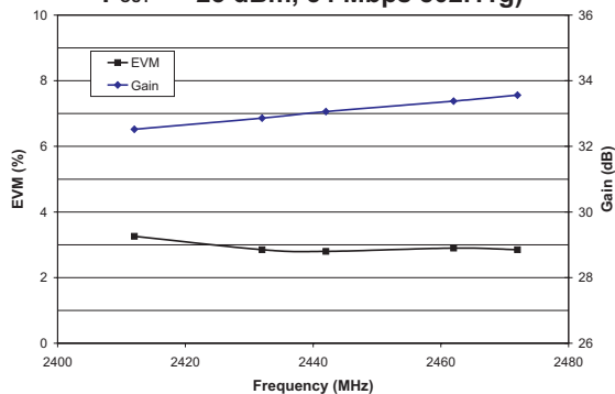
Figure 4: EVM and Gain vs. Frequency ( T_A = +25^\circ\text{C} , V_{CC} = +5\text{ V} , V_{REF} = +2.85\text{ V} , P_{OUT} = +25\text{ dBm} , 54 Mbps 802.11g)
