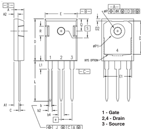
TO-247 Outline
