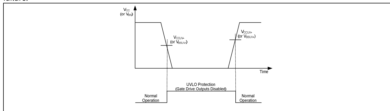
Figure 10 UVLO protection
