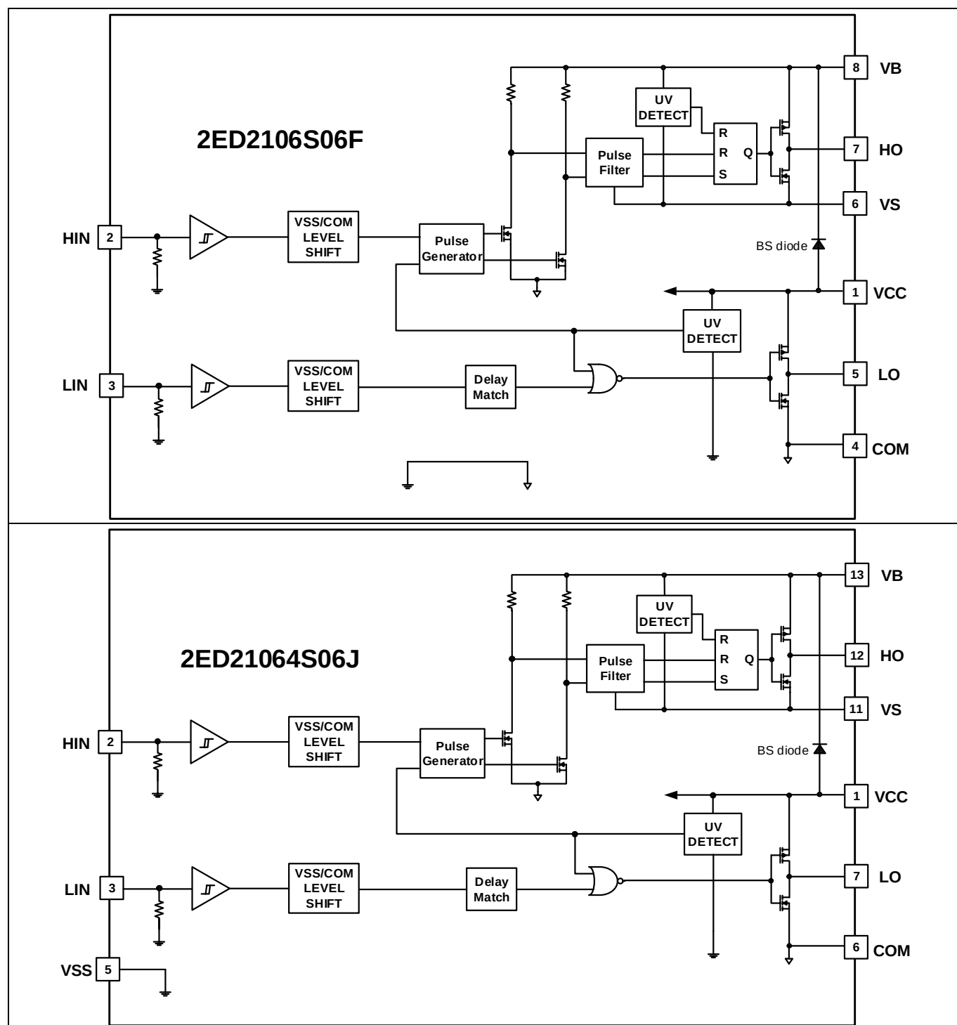
Figure 2 Block diagrams
