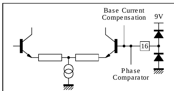
Figure 15 : Pin 16 Configuration
