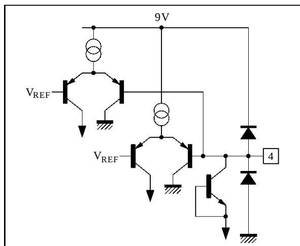
Figure 6 : Pin 4 Configuration
