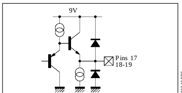
Figure 16 : Pins 17 - 18 - 19 Configuration
