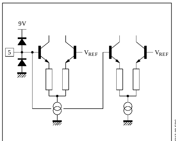
Figure 7 : Pin 5 Configuration
