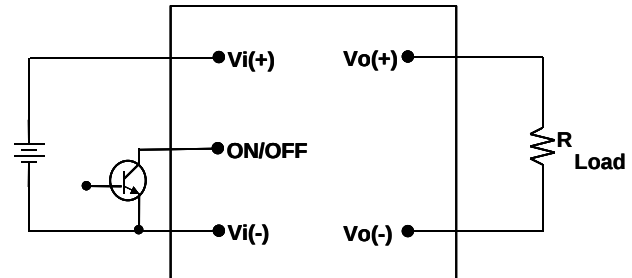
Figure 17: Remote on/off implementation
