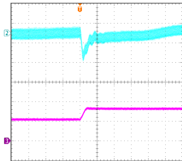
Figure 10: Output voltage response to step-change in load current (50%-75% of I_{o, \max} ; di/dt = 0.1A/\mu s , V_{in}=48V ). Load cap: 10\mu F , tantalum capacitor and 1\mu F ceramic capacitor. Top Trace: V_{out} (200mV/div, 200us/div); Bottom Trace: I_o (15A/div, 200us/div). Scope measurement should be made using a BNC cable (length shorter than 20 inches). Position the load between 51 mm to 76 mm (2 inches to 3 inches) from the module..
