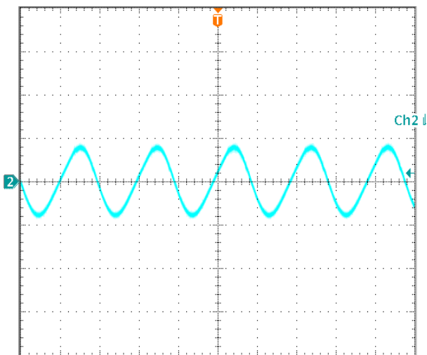
Figure 15: Output voltage ripple at nominal input voltage and rated load current (50 mV/div, 2 \mu\text{s}/\text{div} ) Load capacitance: 1\mu\text{F} ceramic capacitor and 10\mu\text{F} tantalum capacitor. Bandwidth: 20 MHz. Scope measurements should be made using a BNC cable (length shorter than 20 inches). Position the load between 51 mm to 76 mm (2 inches to 3 inches) from the module.
