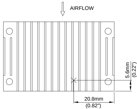
Figure 24: * Hot spot temperature measured point. the allowed maximum hot spot temperature is defined at 100 °C
