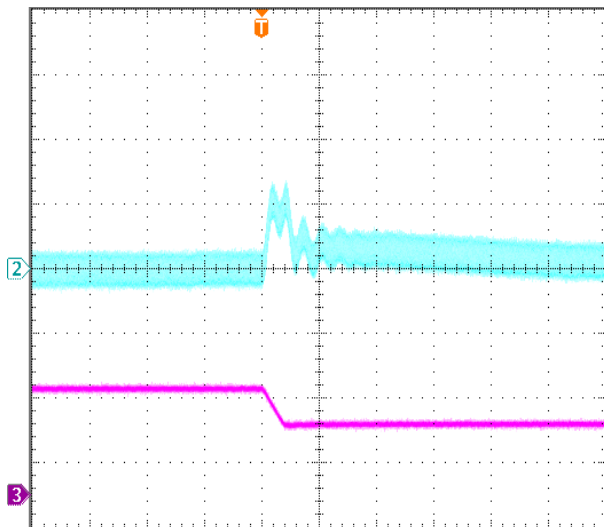
Figure 9: Output voltage response to step-change in load current (75%-50% of I_{o, \max} ; di/dt = 0.1A/\mu s , V_{in}=48V ). Load cap: 10\mu F , tantalum capacitor and 1\mu F ceramic capacitor. Top Trace: V_{out} (200mV/div, 200us/div); Bottom Trace: I_o (15A/div, 200us/div). Scope measurement should be made using a BNC cable (length shorter than 20 inches). Position the load between 51 mm to 76 mm (2 inches to 3 inches) from the module..
