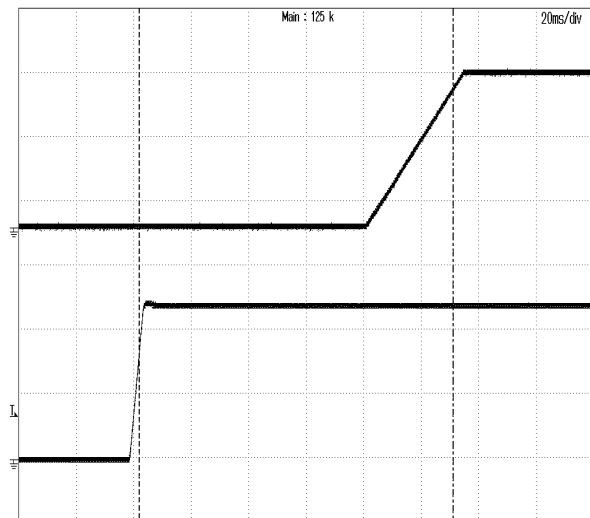
Figure 7: Turn-on transient at zero load current (10 ms/div). V_{in}=48V . Top Trace: V_{out} , 5V/div; Bottom Trace: input voltage, 30V/div
