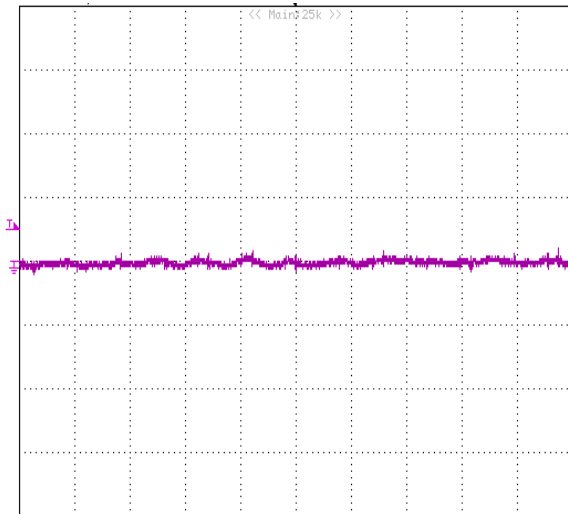
Figure 13: Input reflected ripple current, i_s , through a 12\mu\text{H} source inductor at nominal input voltage and rated load current (20 mA/div, 5 \mu\text{s}/\text{div} ).
