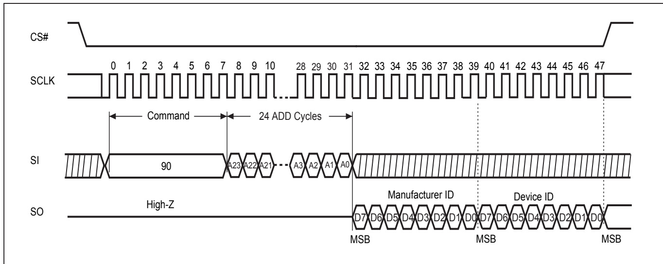
Figure 34. Read Electronic Manufacturer & Device ID (REMS) Sequence (Command 90 or EF or DF or CF)
