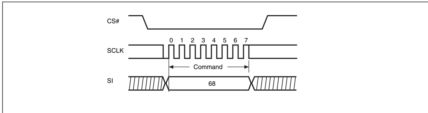
Figure 35. Write Protection Selection (WPSEL) Sequence (Command 68)
