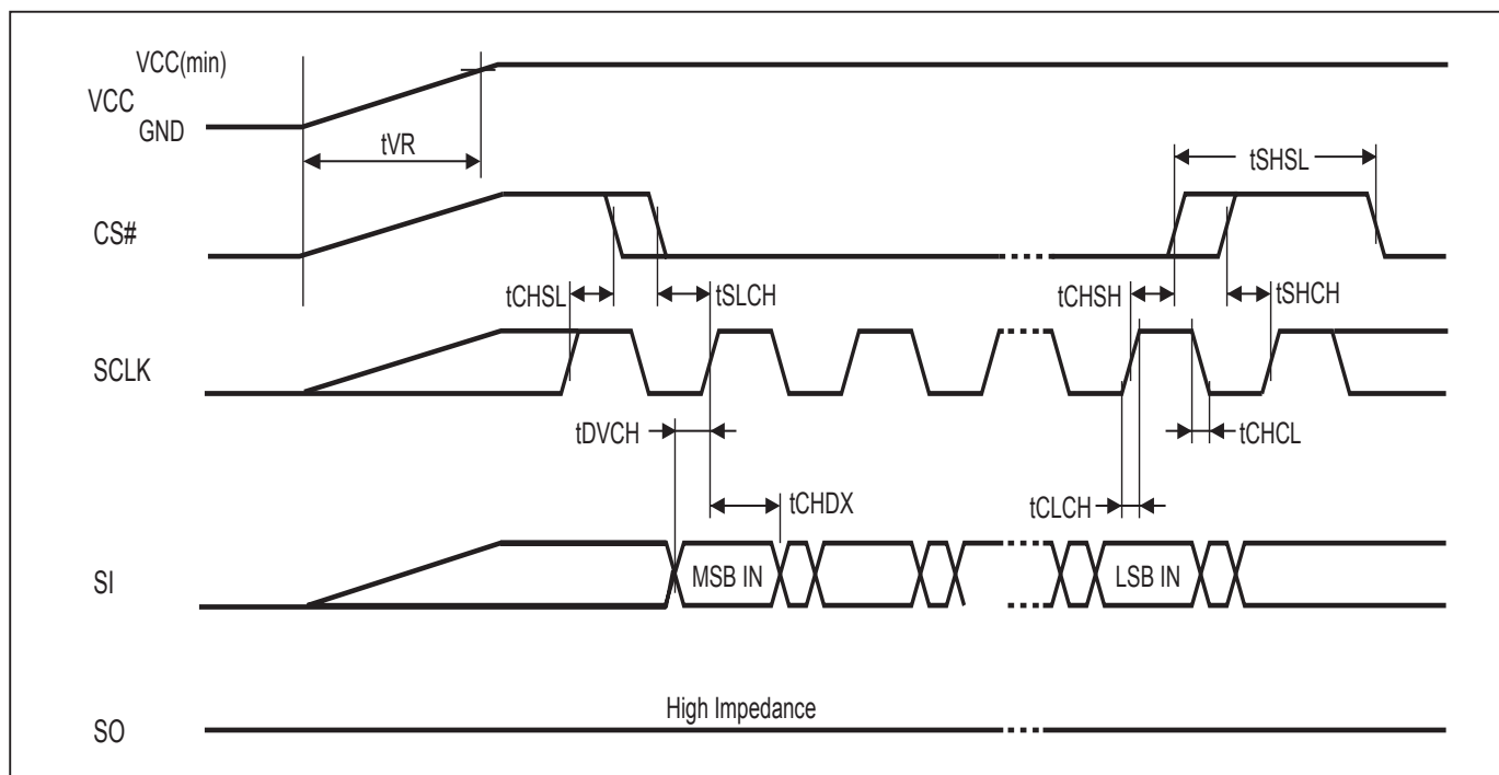
Figure 40. AC Timing at Device Power-Up
