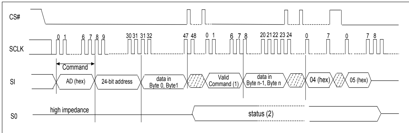
Figure 30. Continously Program (CP) Mode Sequence with Hardware Detection (Command AD)
