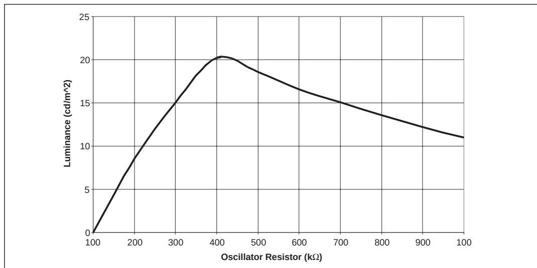
Figure 13. Luminance (cd/m²) vs R_{osc}
