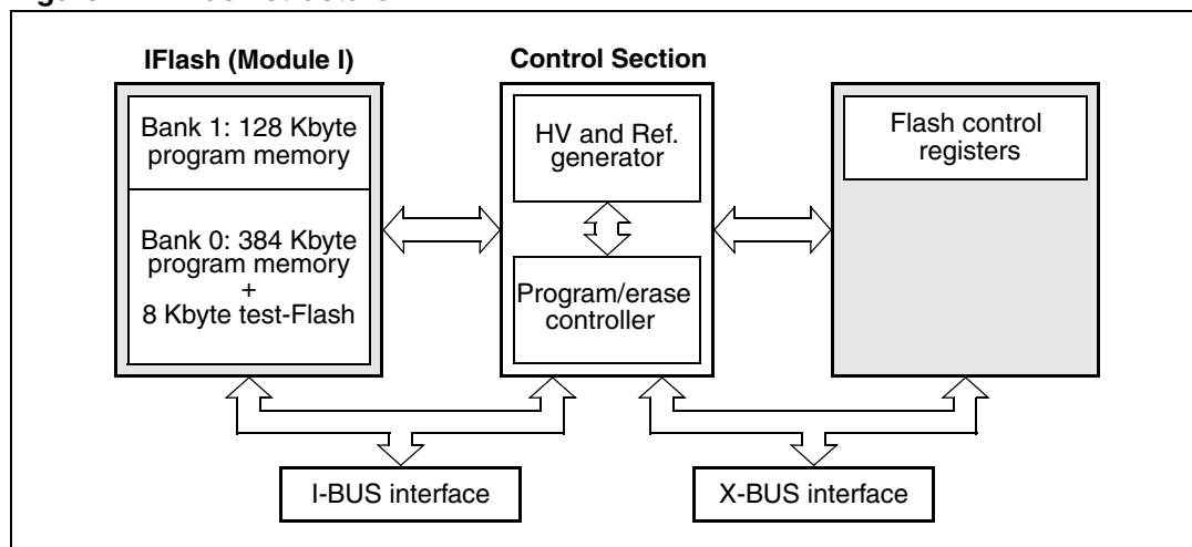
Figure 4. Flash structure
