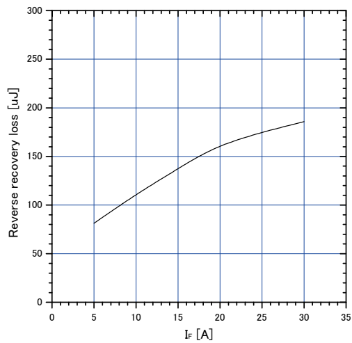
Graph.15 Typical reverse recovery loss vs. I_F T_J=175^\circ\text{C} , V_{CC}=400\text{V} , L=500\mu\text{H} V_{GE}=15\text{V} , R_G=10\Omega
