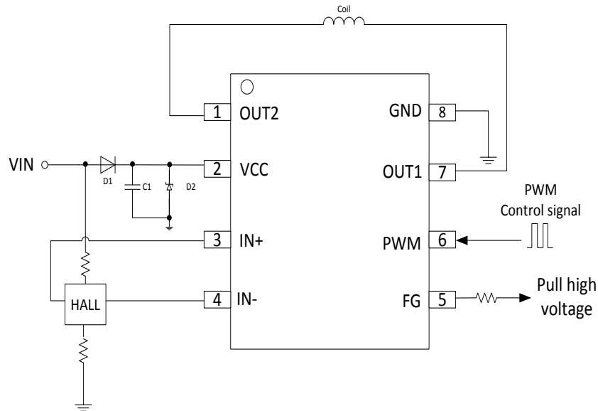
Figure 4. Typical Application
