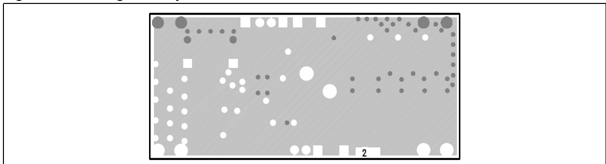
Figure 24. Signal-ground layer
