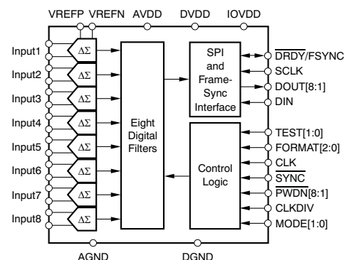
ADS1278
