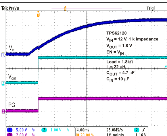
Figure 35. Startup From a High-Impedance Source
