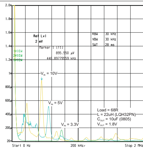
Figure 27. TPS62120 Spurious Output Noise COUT = 10µF
