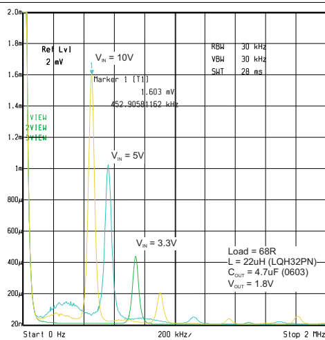
Figure 26. TPS62120 Spurious Output Noise COUT = 4.7µF
