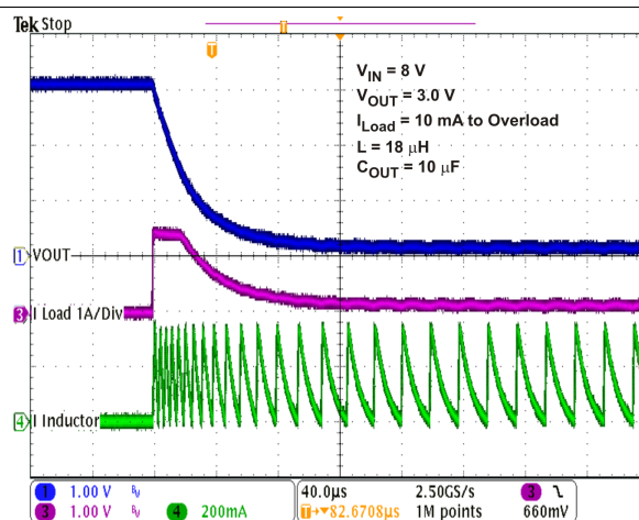
Figure 33. Output Overload Protection
