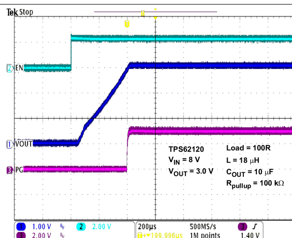
Figure 31. Power Good Output During Startup
