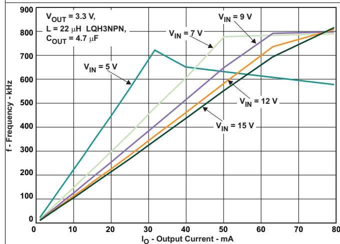
Figure 5. Switch Frequency vs Output Current I_{OUT} ( V_{OUT} = 3.3\text{ V} )
