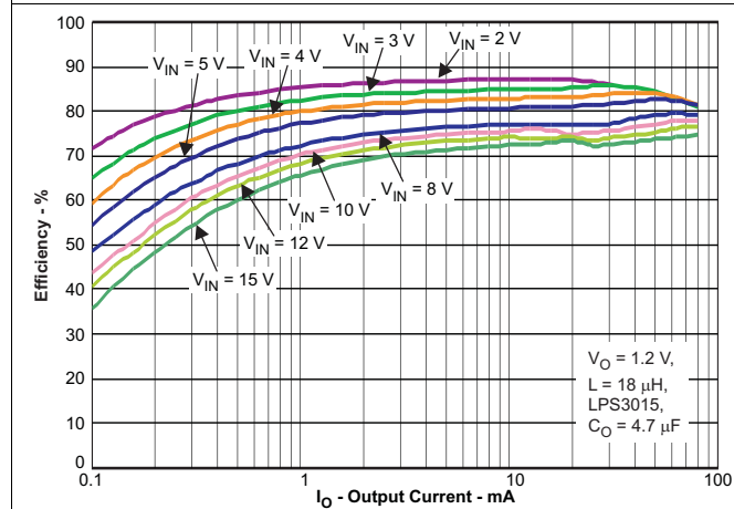
Figure 16. Efficiency vs Output Current I_{OUT} ( V_{OUT} = 1.2 V)
