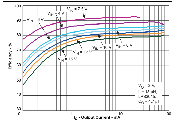
Figure 14. Efficiency vs Output Current I_{OUT} ( V_{OUT} = 2 V)
