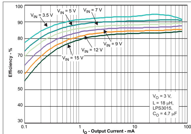
Figure 12. Efficiency vs Output Current I_{OUT} ( V_{OUT} = 3 V)
