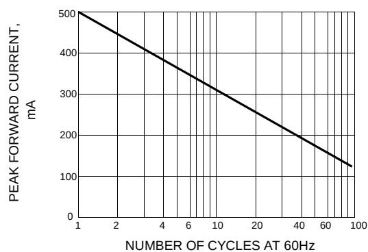
FIG.3 - MAXIMUM PEAK FORWARD CURRENT
