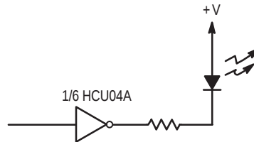
LED Driver
