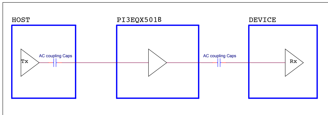
PI3EQX501B Application Schematics
