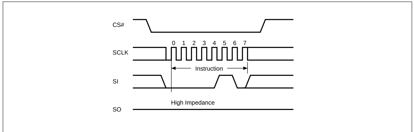
Figure 12. Write Enable (WREN) Instruction Sequence
