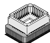
100-pin Ceramic MQFP
