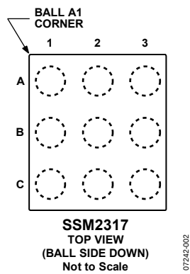
Figure 2. Pin Configuration
