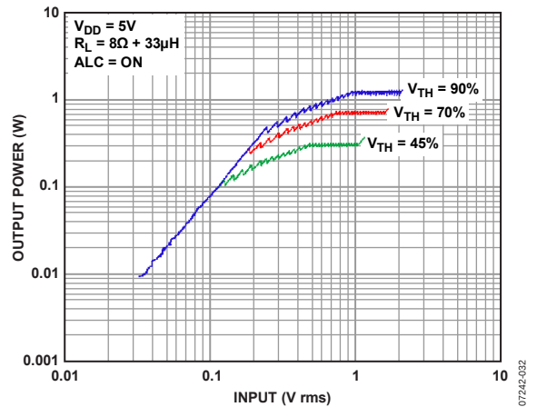
Figure 32. Input/Output Characteristic, V_{DD} = 5V , ALC = On
